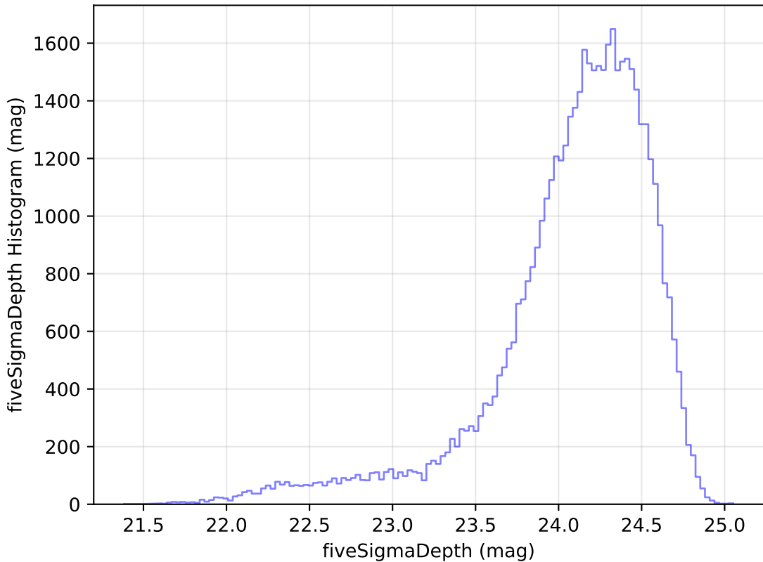
ddf_loaded_half_fl8_v3.4_10yrs Yr 1 r band: fiveSigmaDepth Histogram
