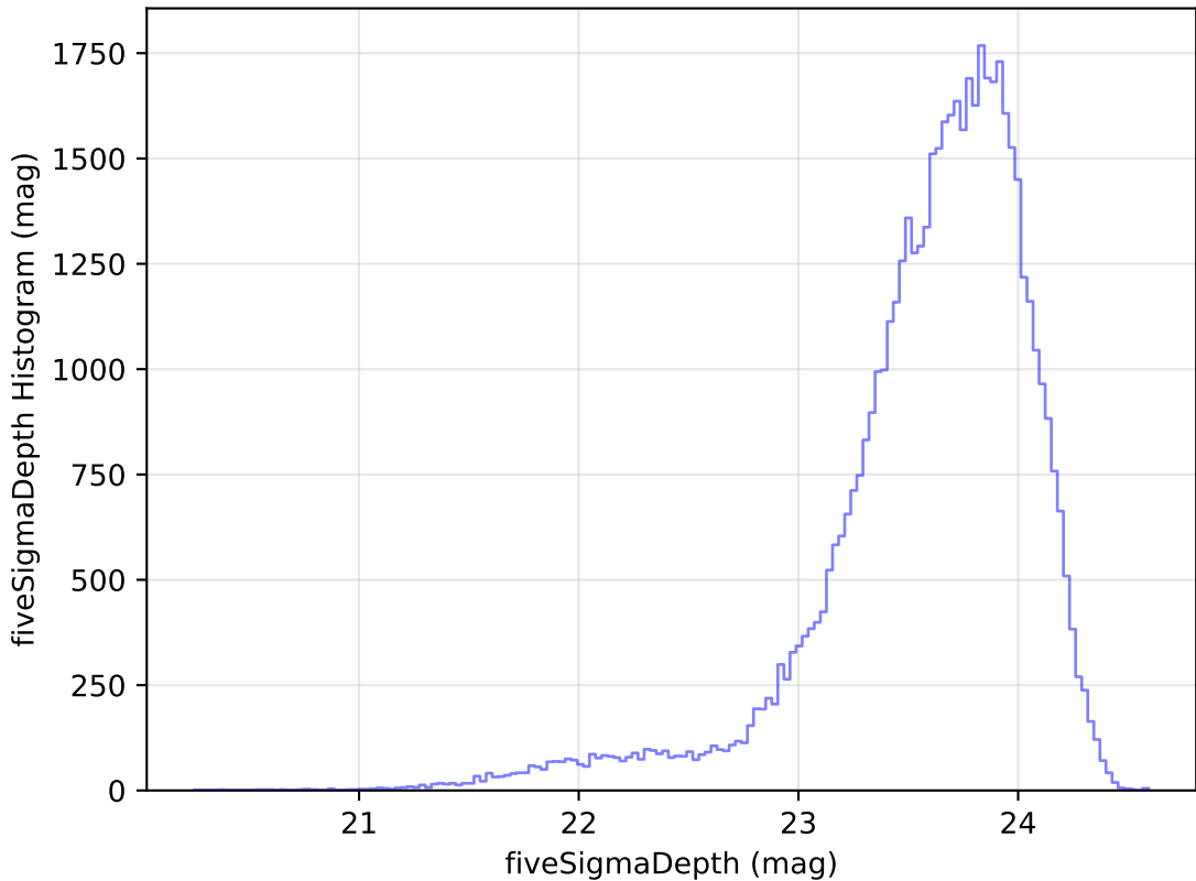
ddf_loaded_half_fl8_v3.4_10yrs Yr 1 i band: fiveSigmaDepth Histogram
