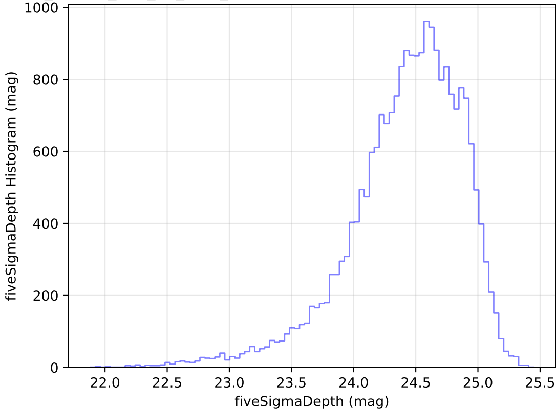
ddf_loaded_half_fl8_v3.4_10yrs Yr 1 g band: fiveSigmaDepth Histogram
