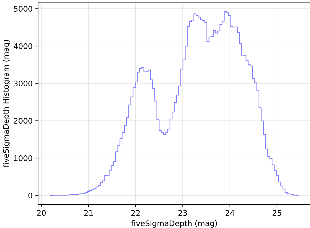
ddf_loaded_half_fl8_v3.4_10yrs Yr 1 all bands: fiveSigmaDepth Histogram
