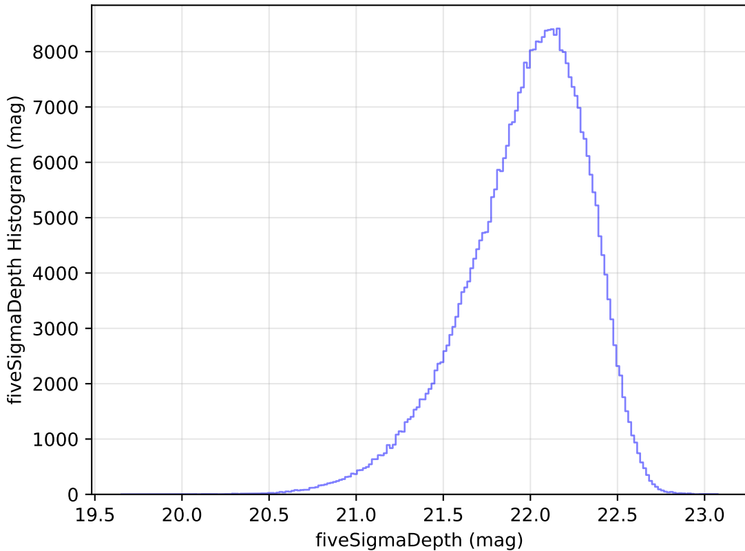
ddf_loaded_half_fl8_v3.4_10yrs WFD y band: fiveSigmaDepth Histogram
