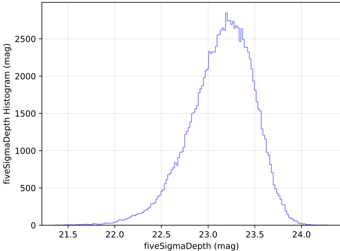
ddf_loaded_half_fl8_v3.4_10yrs WFD u band: fiveSigmaDepth Histogram
