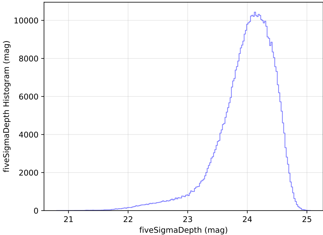
ddf_loaded_half_fl8_v3.4_10yrs WFD r band: fiveSigmaDepth Histogram
