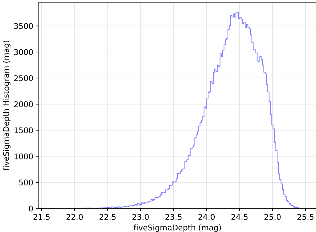
ddf_loaded_half_fl8_v3.4_10yrs WFD g band: fiveSigmaDepth Histogram
