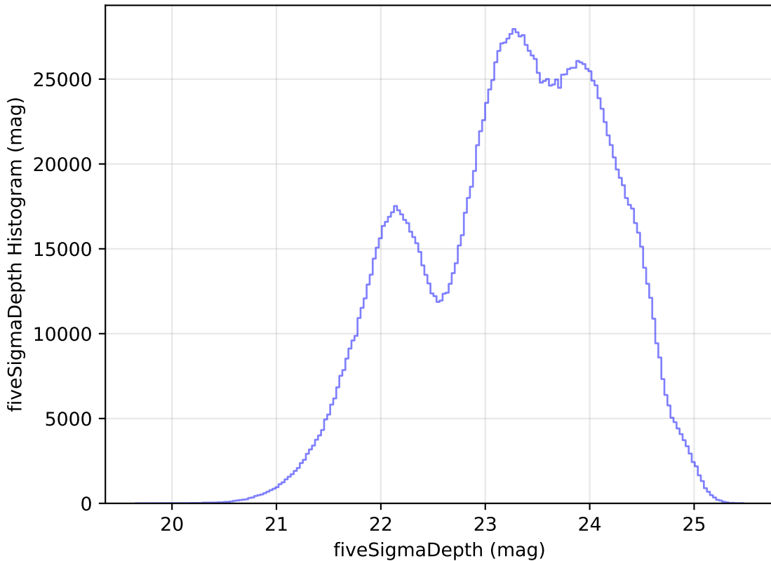
ddf_loaded_half_fl8_v3.4_10yrs WFD all bands: fiveSigmaDepth Histogram
