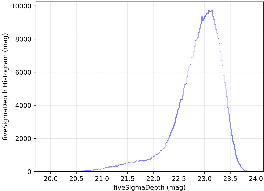
ddf_loaded_half_fl8_v3.4_10yrs All sky z band: fiveSigmaDepth Histogram
