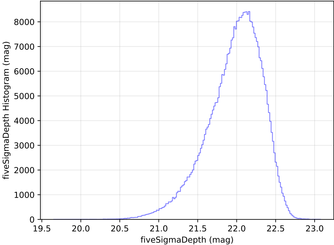
ddf_loaded_half_fl8_v3.4_10yrs All sky y band: fiveSigmaDepth Histogram
