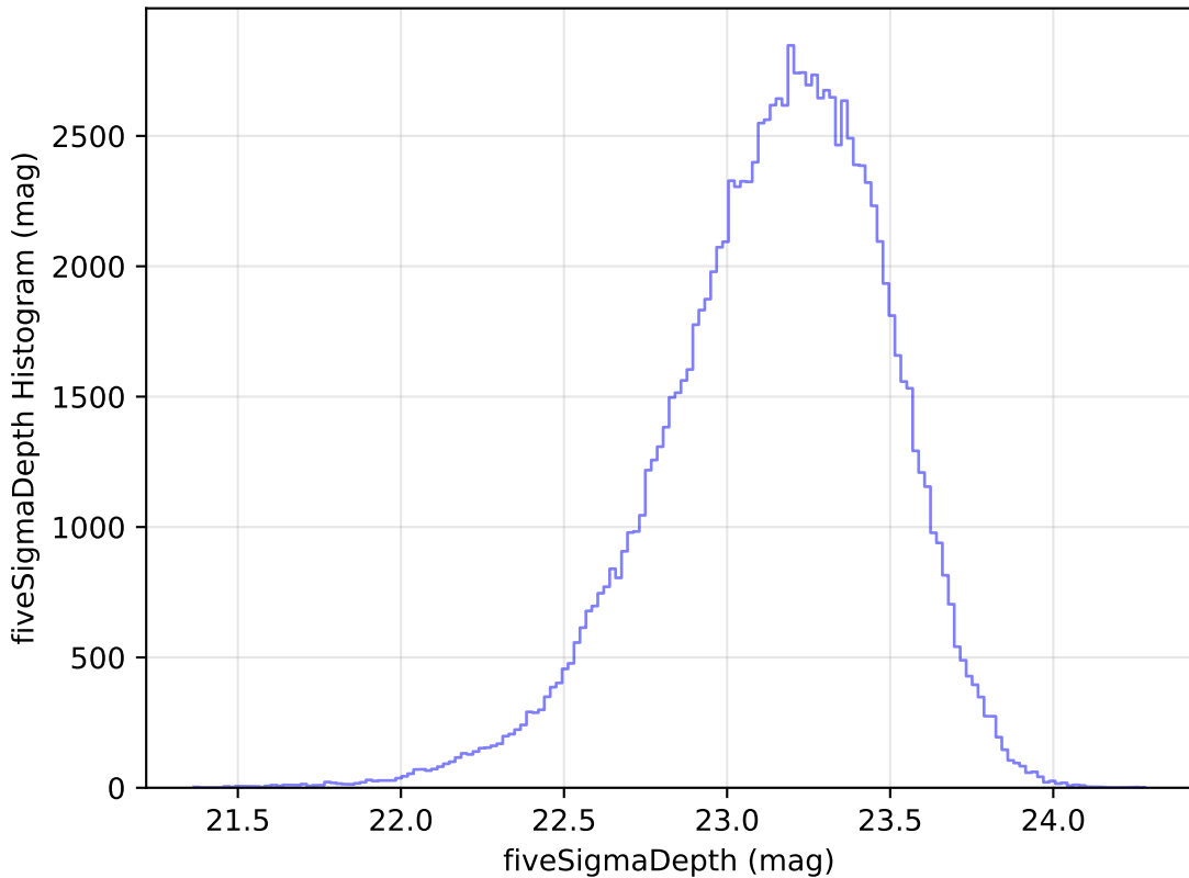
ddf_loaded_half_fl8_v3.4_10yrs All sky u band: fiveSigmaDepth Histogram
