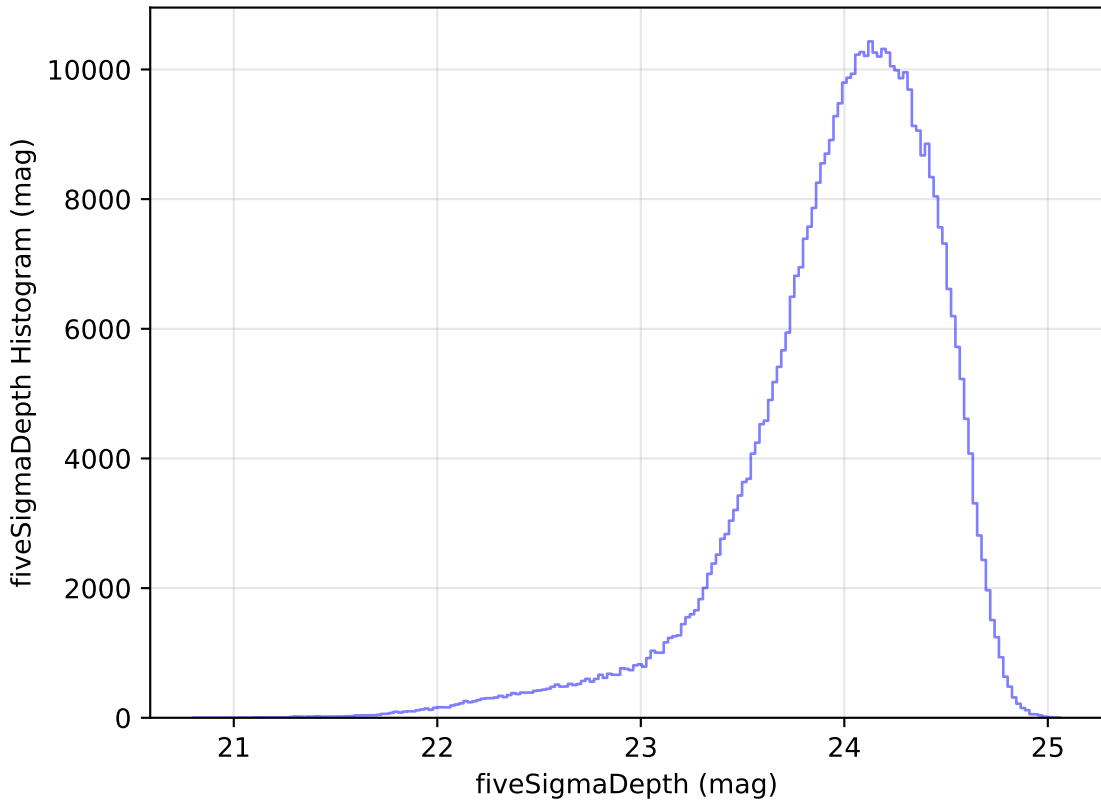
ddf_loaded_half_fl8_v3.4_10yrs All sky r band: fiveSigmaDepth Histogram
