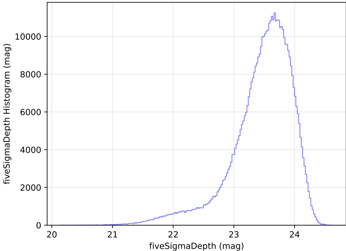
ddf_loaded_half_fl8_v3.4_10yrs All sky i band: fiveSigmaDepth Histogram
