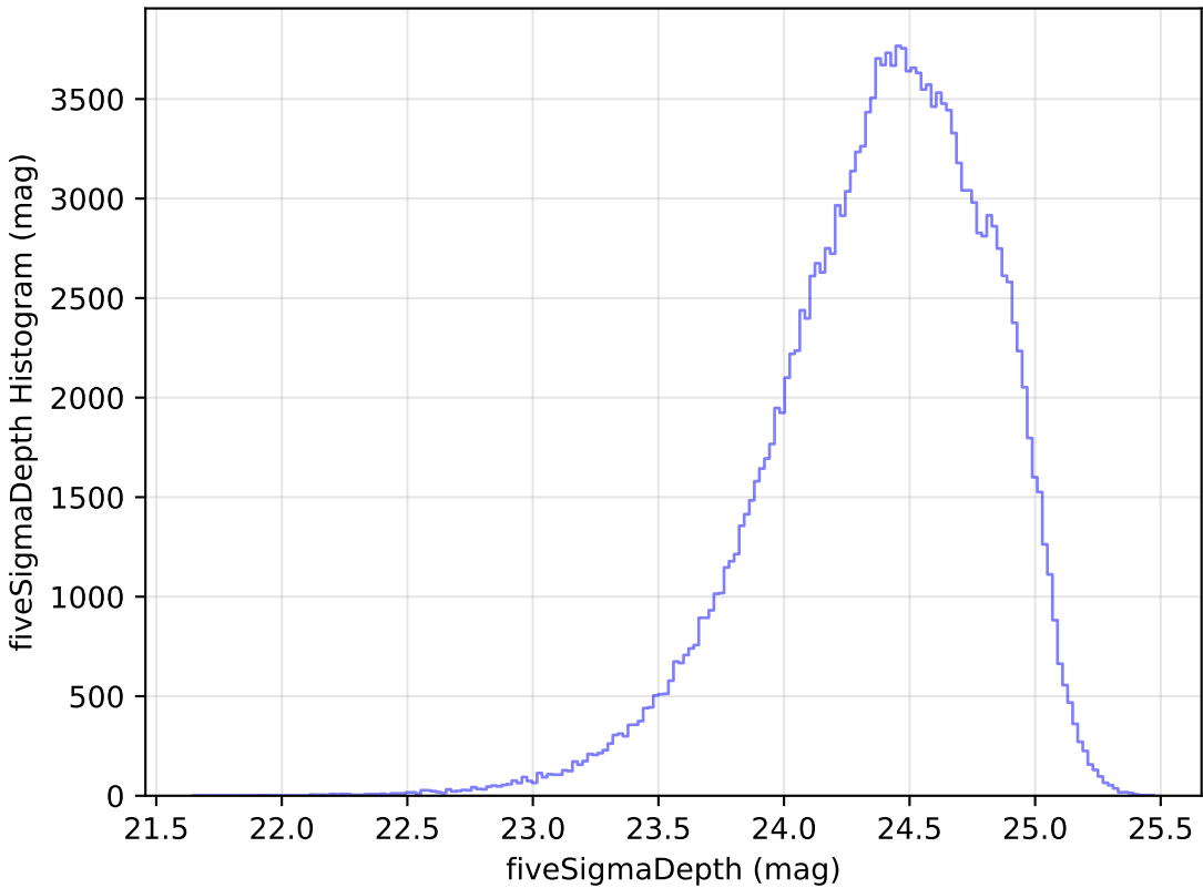
ddf_loaded_half_fl8_v3.4_10yrs All sky g band: fiveSigmaDepth Histogram
