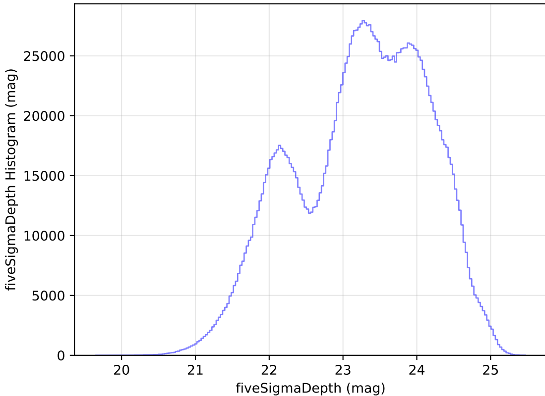
ddf_loaded_half_fl8_v3.4_10yrs All sky all bands: fiveSigmaDepth Histogram
