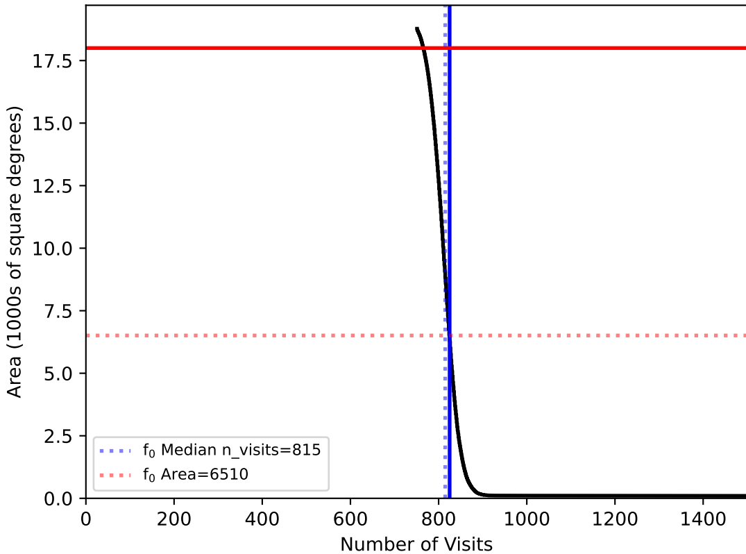
ddf_loaded_half_fl8_v3.4_10yrs WFD: fO
