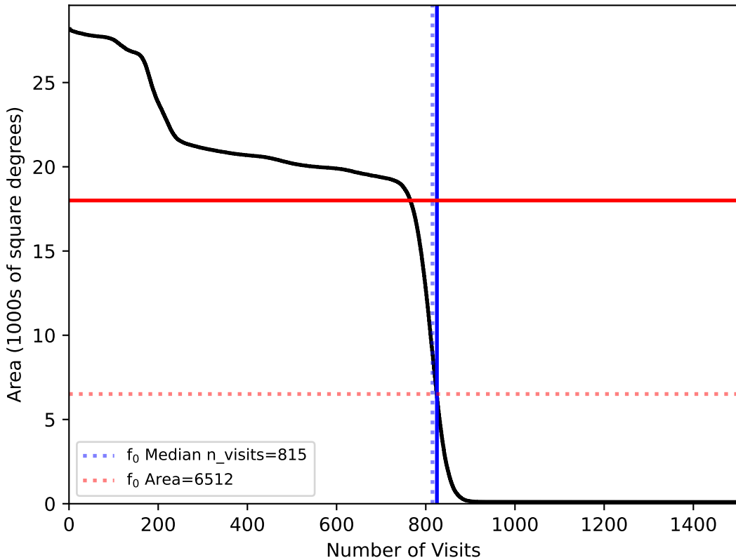
ddf_loaded_half_fl8_v3.4_10yrs All sky: fO
