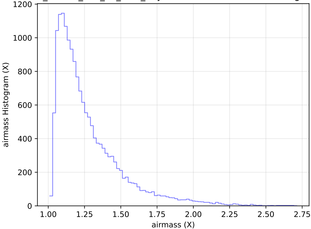
ddf_loaded_half_fl8_v3.4_10yrs Yr 1 u band: airmass Histogram
