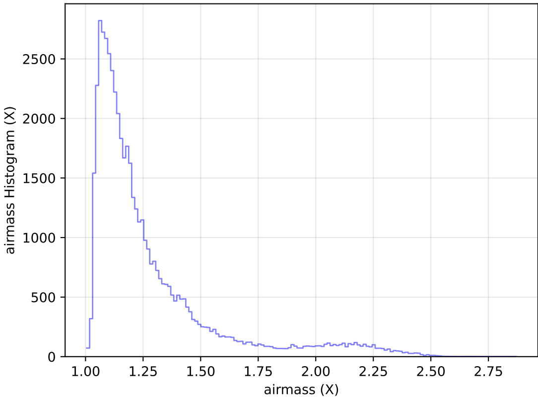
ddf_loaded_half_fl8_v3.4_10yrs Yr 1 r band: airmass Histogram
