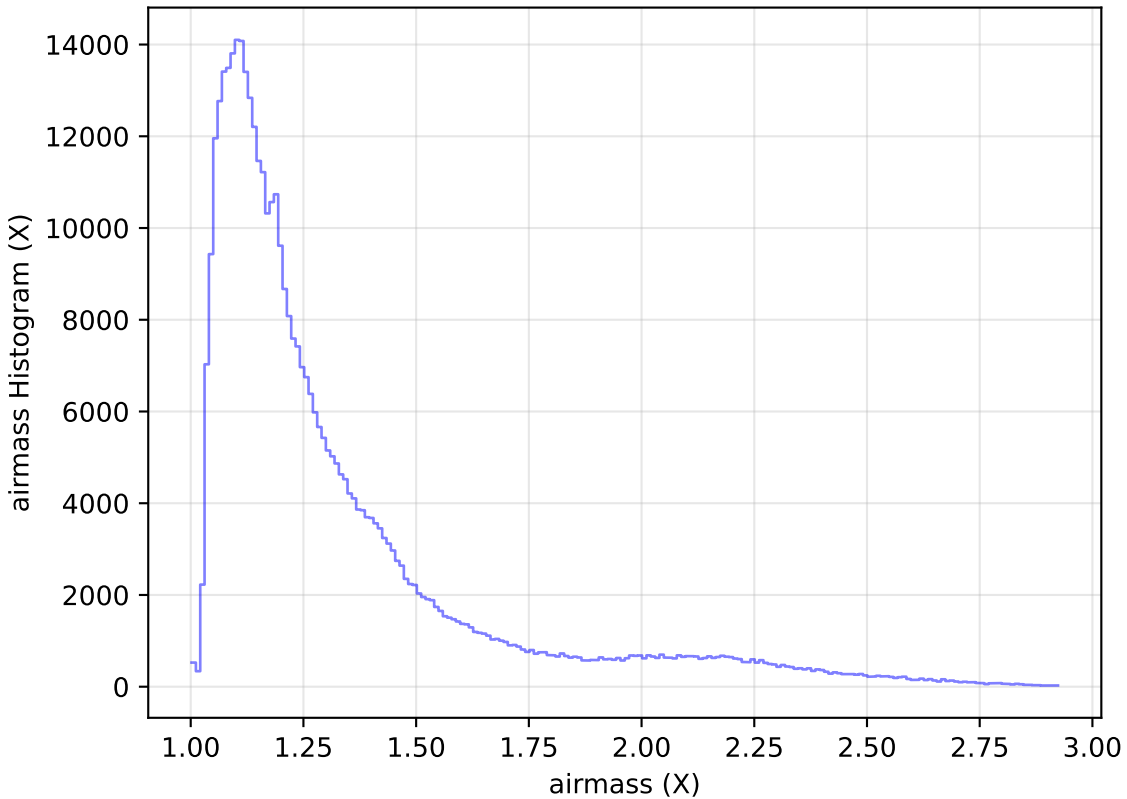
ddf_loaded_half_fl8_v3.4_10yrs WFD z band: airmass Histogram
