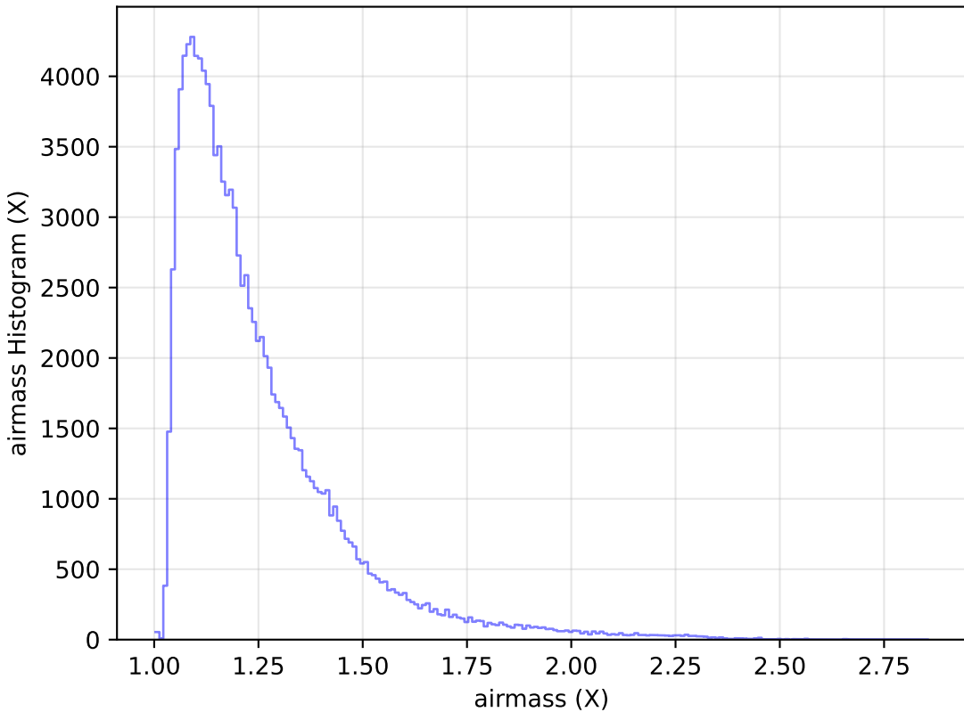
ddf_loaded_half_fl8_v3.4_10yrs WFD u band: airmass Histogram
