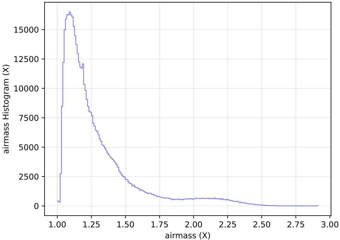
ddf_loaded_half_fl8_v3.4_10yrs WFD r band: airmass Histogram
