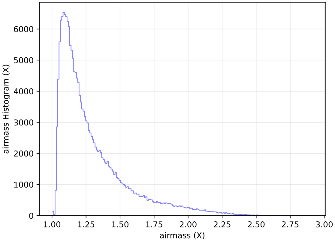
ddf_loaded_half_fl8_v3.4_10yrs WFD g band: airmass Histogram
