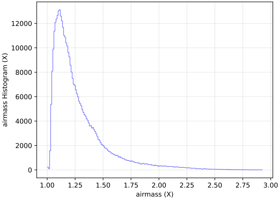
ddf_loaded_half_fl8_v3.4_10yrs All sky y band: airmass Histogram
