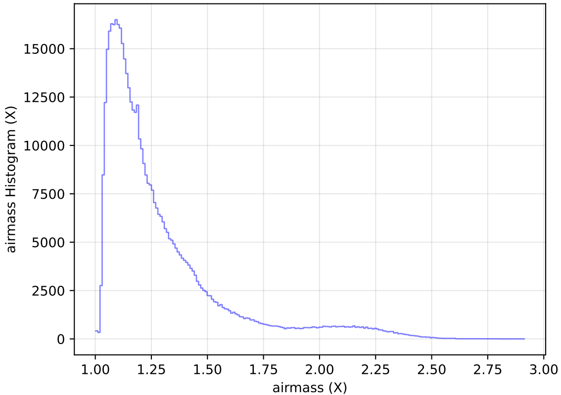
ddf_loaded_half_fl8_v3.4_10yrs All sky r band: airmass Histogram
