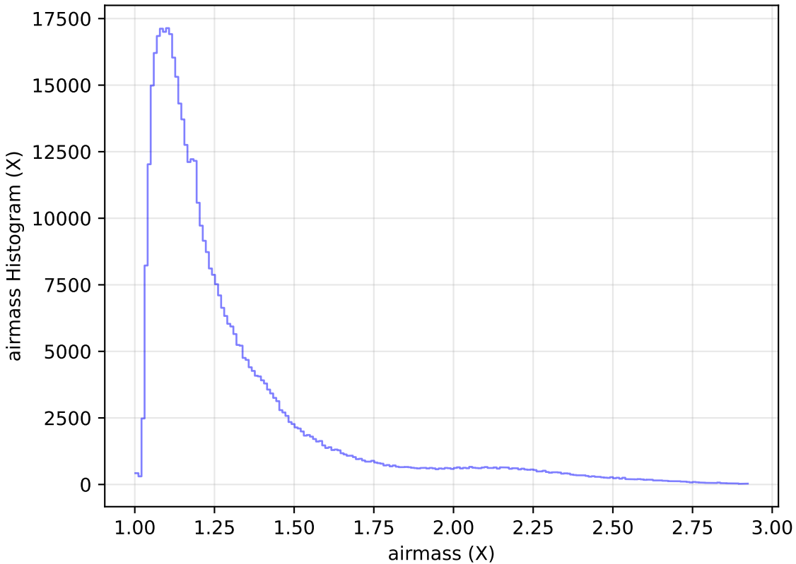
ddf_loaded_half_fl8_v3.4_10yrs All sky i band: airmass Histogram
