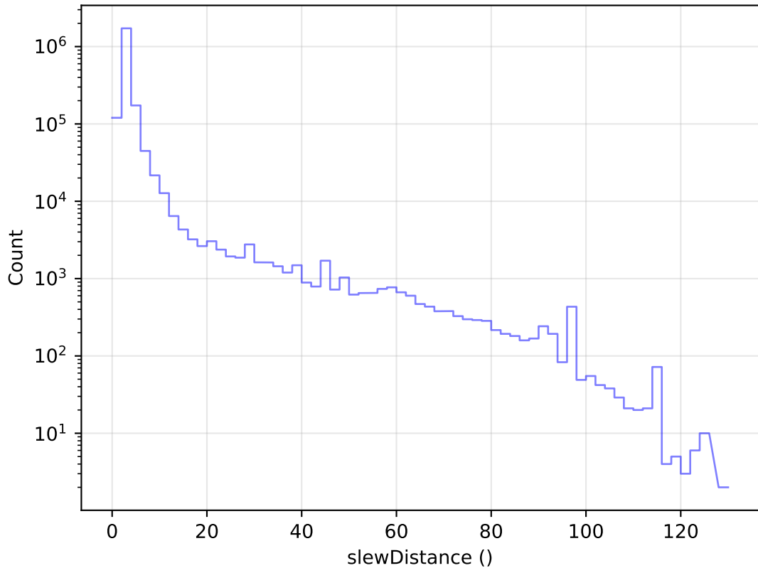
ddf_loaded_half_fl8_v3.4_10yrs All visits: Slew Distance Histogram
