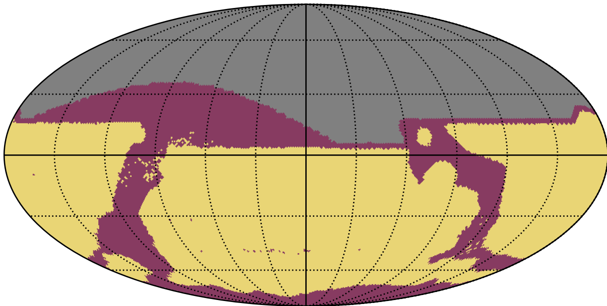
ddf_loaded_half_fl8_v3.4_10yrs All sky: RapidRevisits
