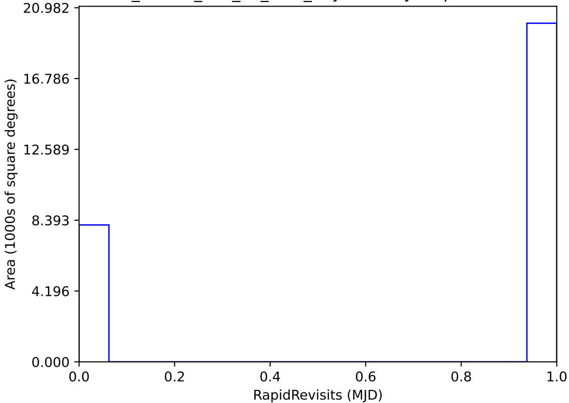
ddf_loaded_half_fl8_v3.4_10yrs All sky: RapidRevisits
