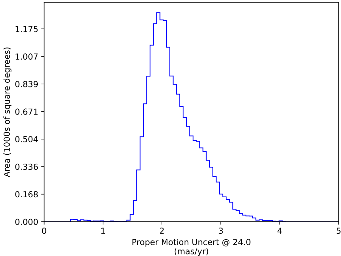
ddf_loaded_half_fl8_v3.4_10yrs WFD: Proper Motion Uncert @ 24.0
