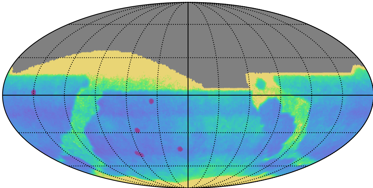
ddf_loaded_half_fl8_v3.4_10yrs All sky: Proper Motion Uncert @ 24.0
