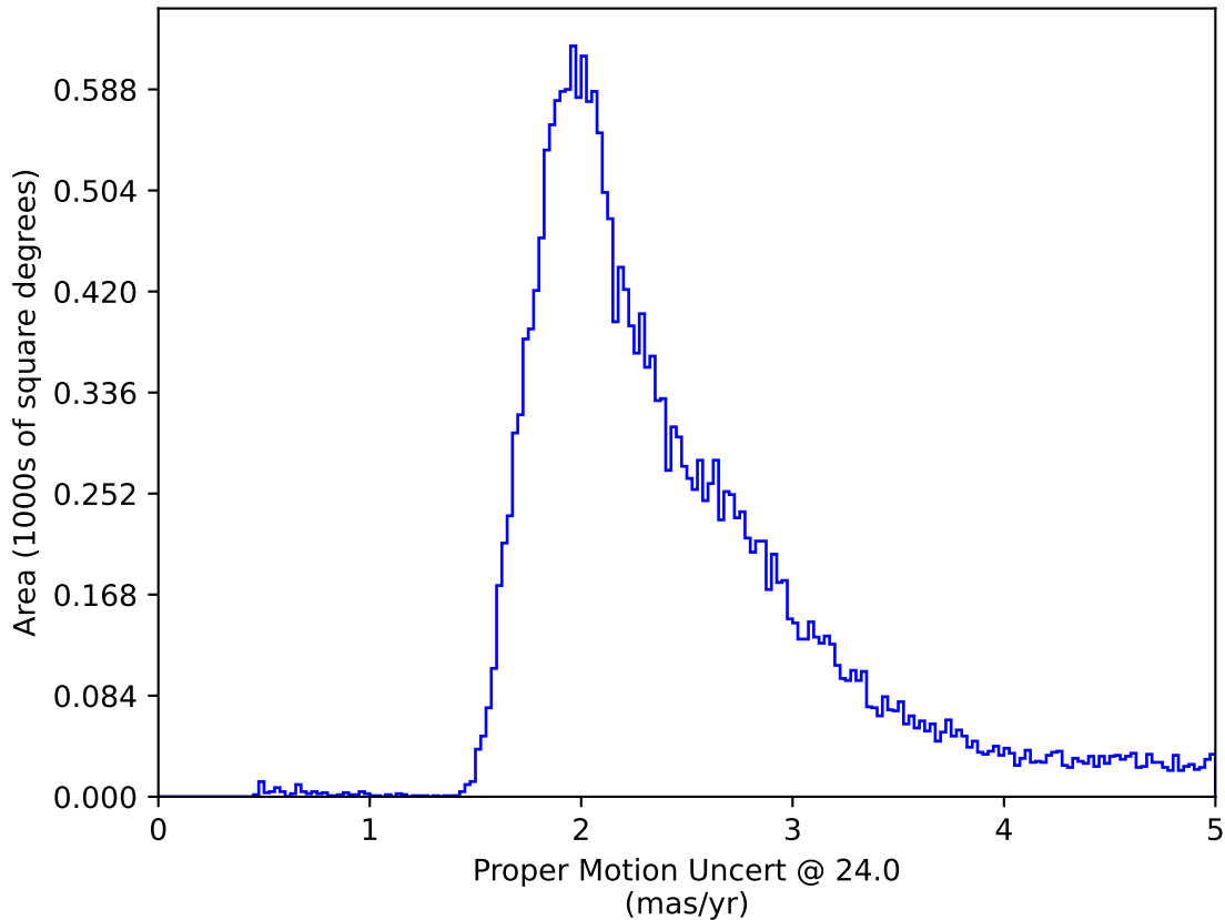
ddf_loaded_half_f18_v3.4_10yrs All sky: Proper Motion Uncert @ 24.0
