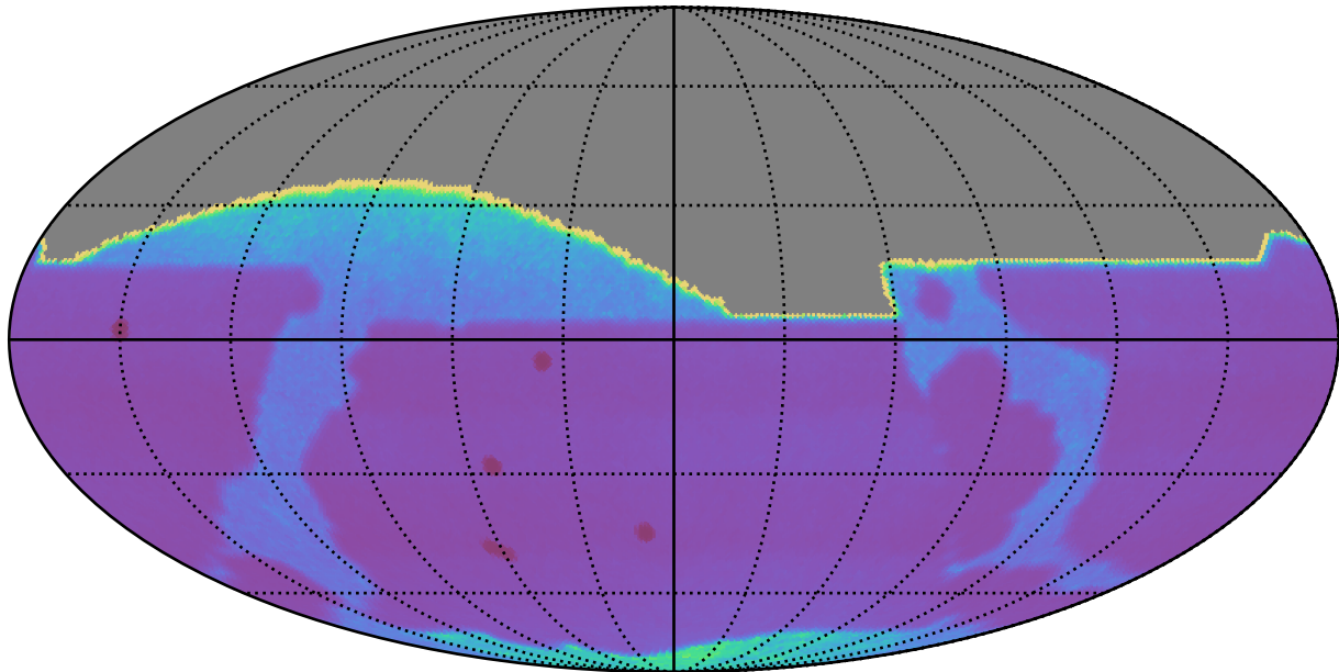
ddf_loaded_half_fl8_v3.4_10yrs All sky: Proper Motion Uncert @ 20.5
