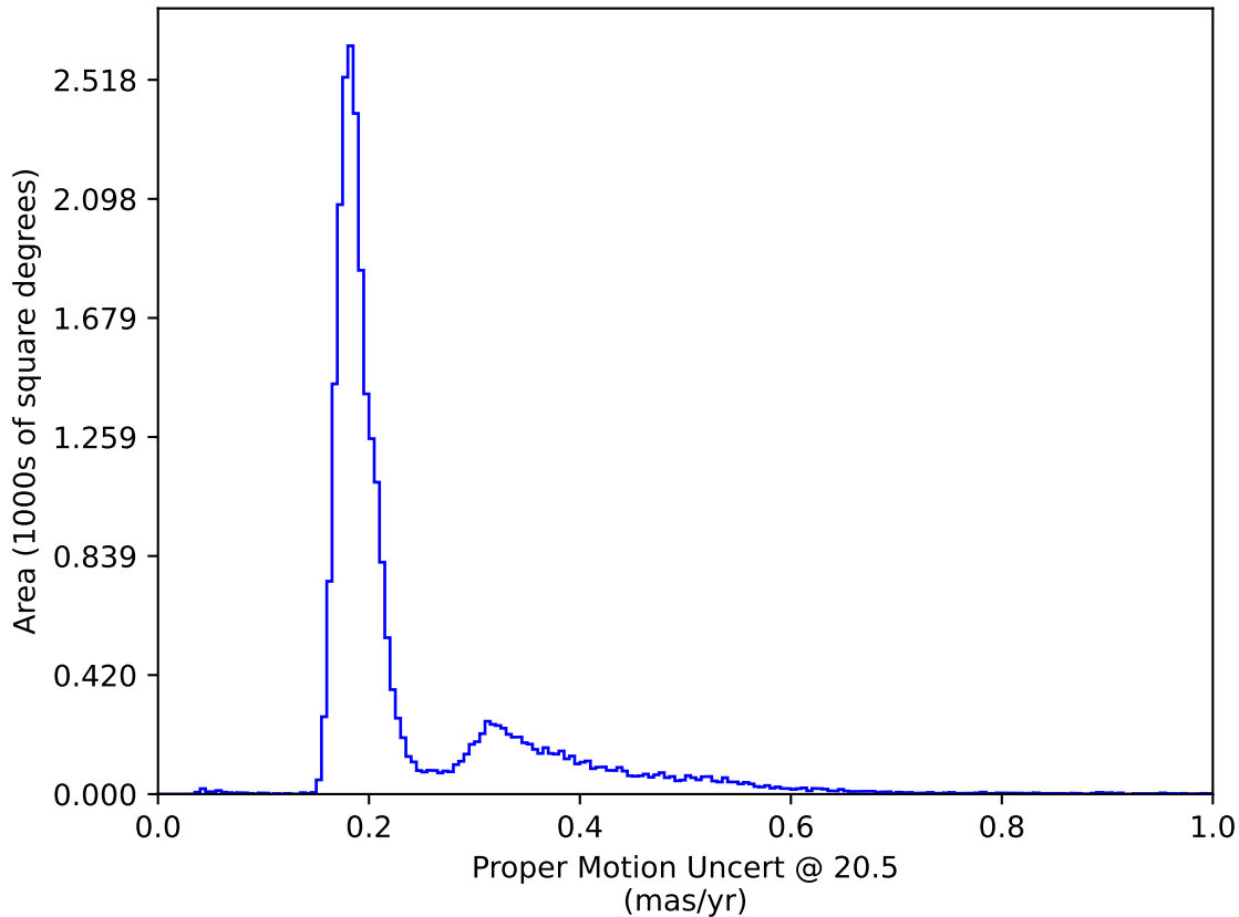
ddf_loaded_half_fl8_v3.4_10yrs All sky: Proper Motion Uncert @ 20.5
