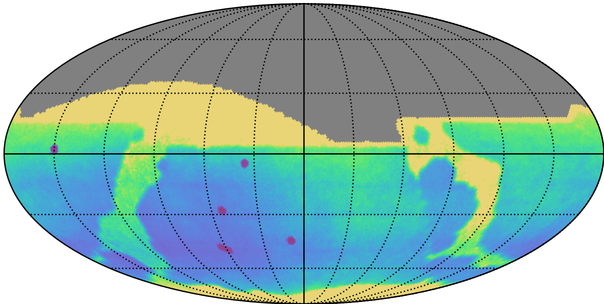
ddf_loaded_half_fl8_v3.4_10yrs All sky: Parallax Uncert @ 24.0
