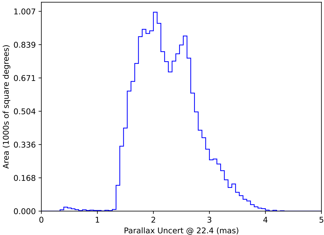
ddf_loaded_half_fl8_v3.4_10yrs WFD: Parallax Uncert @ 22.4
