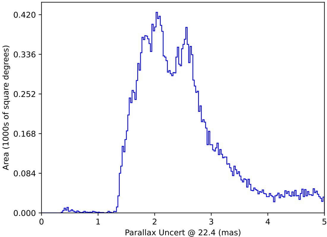
ddf_loaded_half_fl8_v3.4_10yrs All sky: Parallax Uncert @ 22.4
