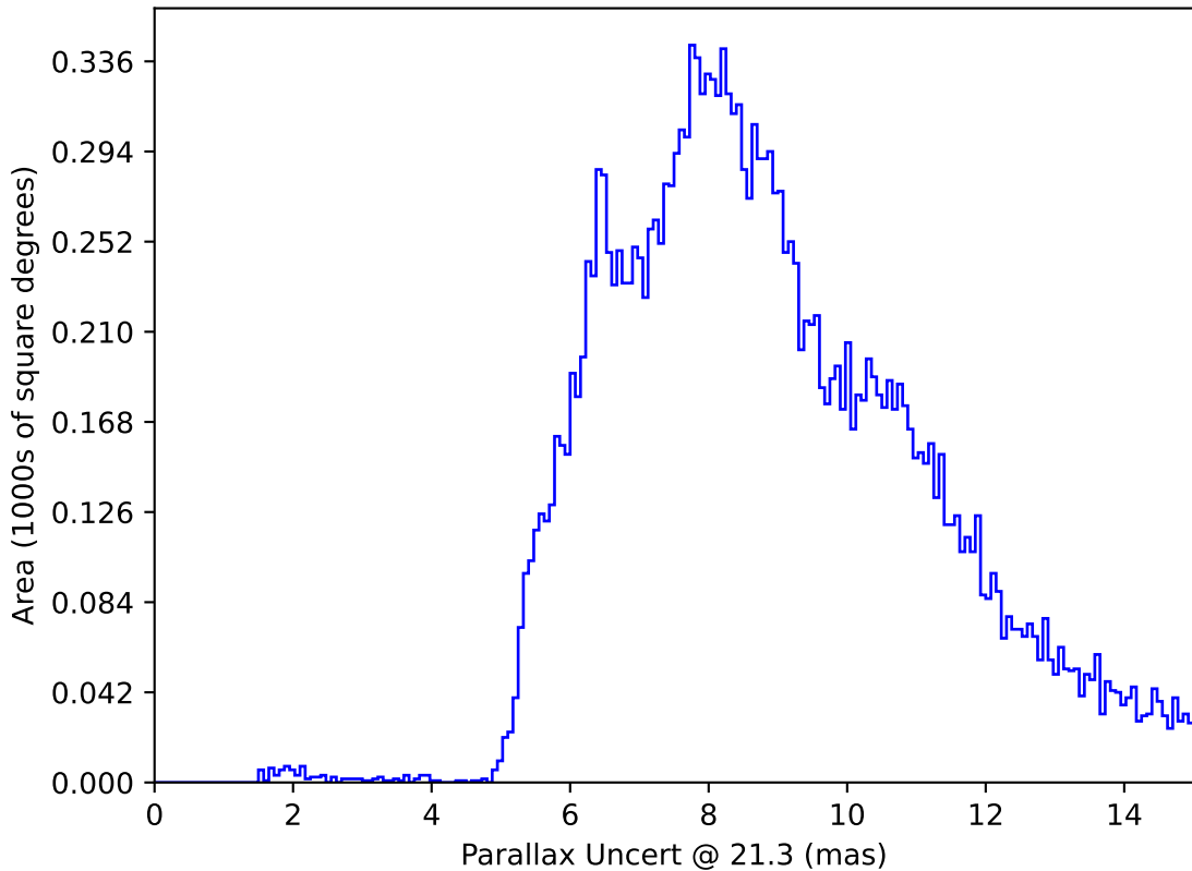
ddf_loaded_half_fl8_v3.4_10yrs All sky y band only: Parallax Uncert @ 21.3
