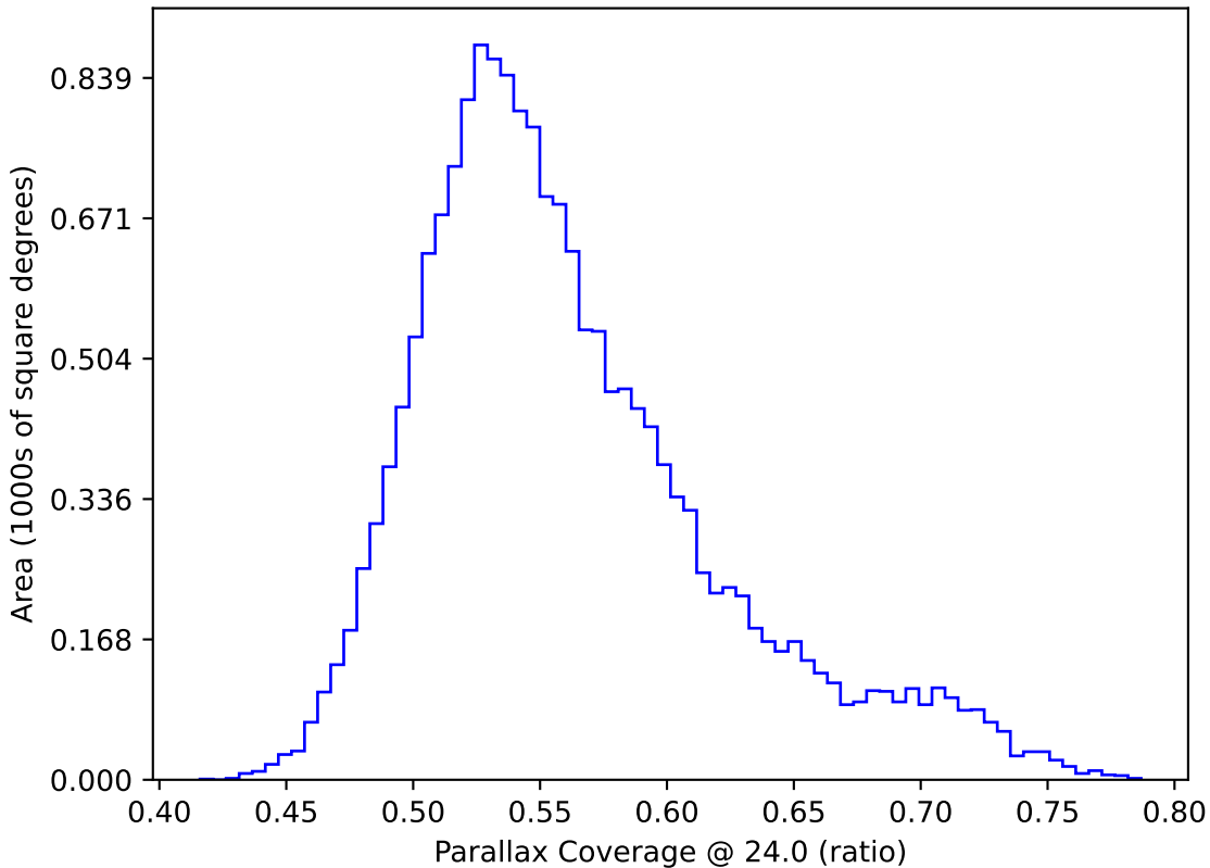
ddf_loaded_half_fl8_v3.4_10yrs WFD: Parallax Coverage @ 24.0
