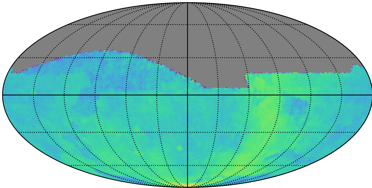
ddf_loaded_half_fl8_v3.4_10yrs All sky: Parallax Coverage @ 24.0
