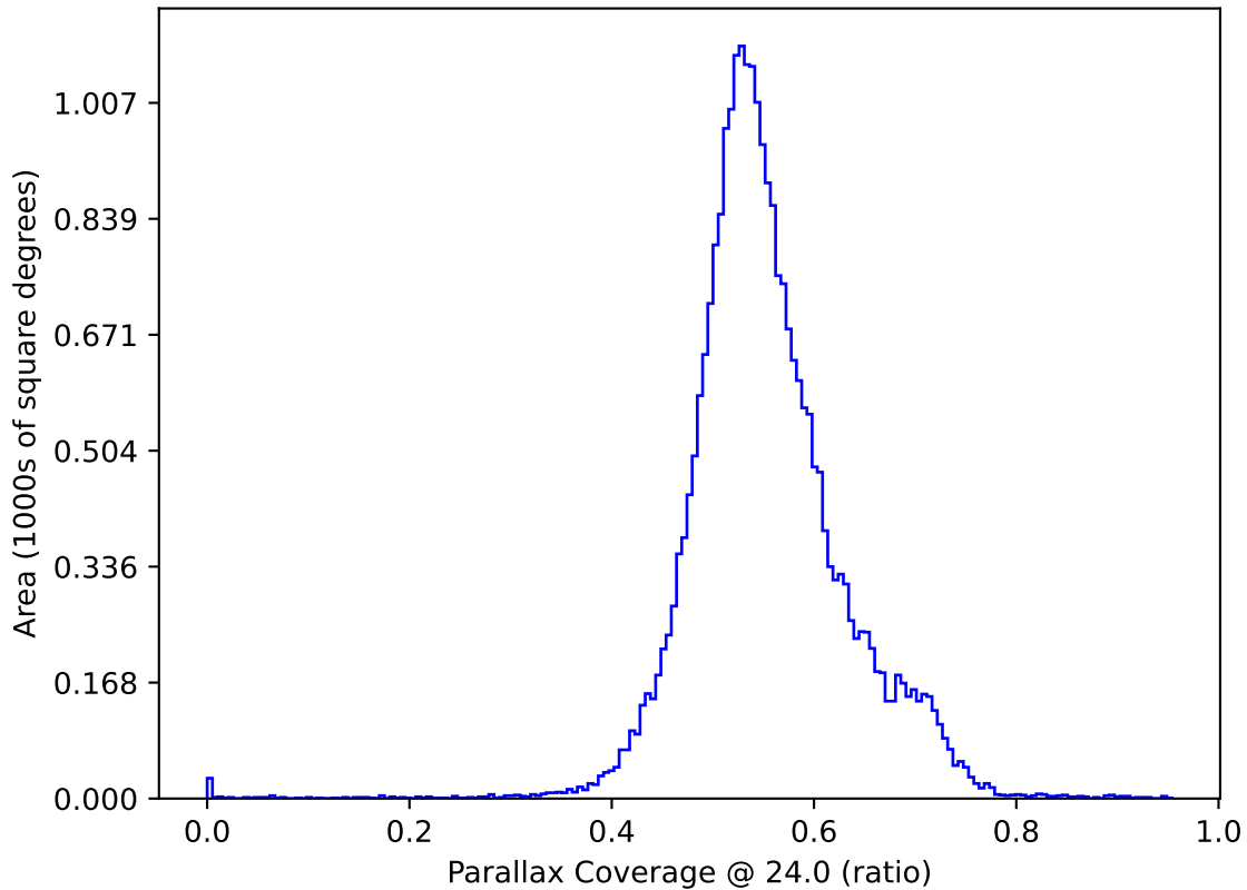
ddf_loaded_half_fl8_v3.4_10yrs All sky: Parallax Coverage @ 24.0
