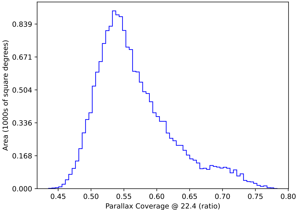
ddf_loaded_half_fl8_v3.4_10yrs WFD: Parallax Coverage @ 22.4
