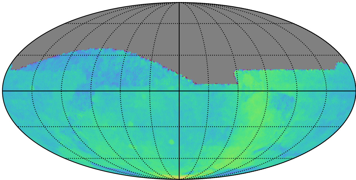
ddf_loaded_half_fl8_v3.4_10yrs All sky: Parallax Coverage @ 22.4
