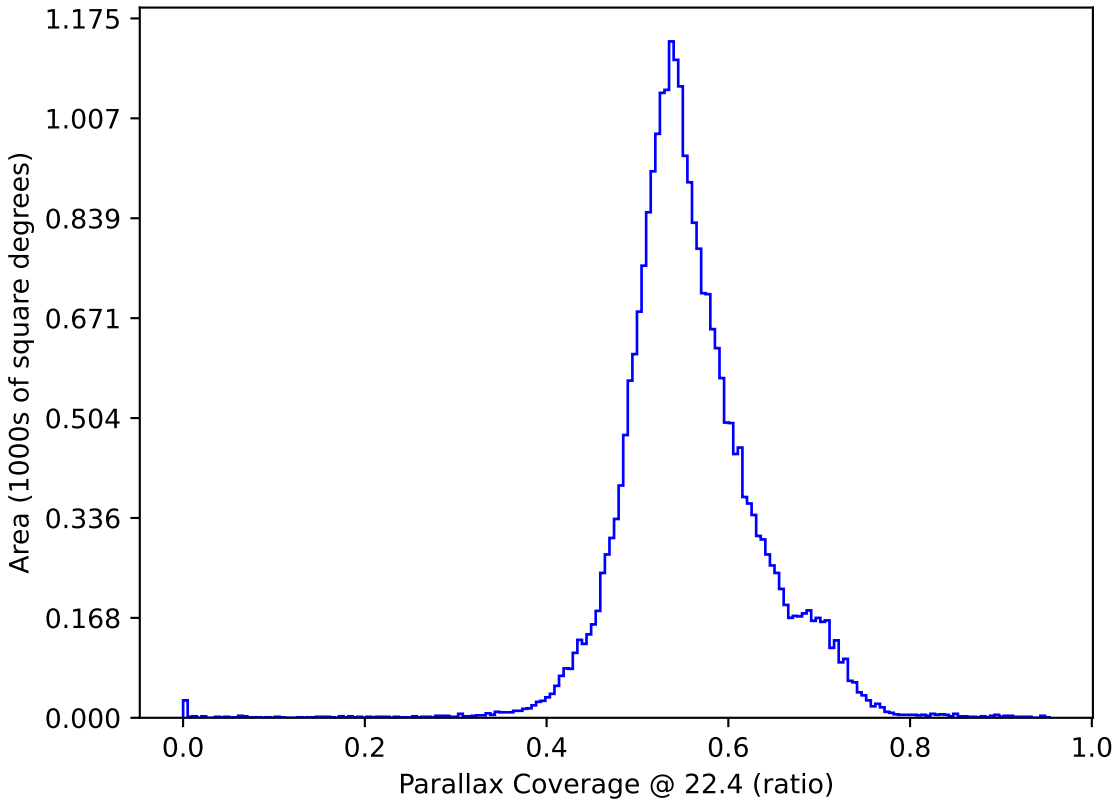
ddf_loaded_half_fi8_v3.4_10yrs All sky: Parallax Coverage @ 22.4
