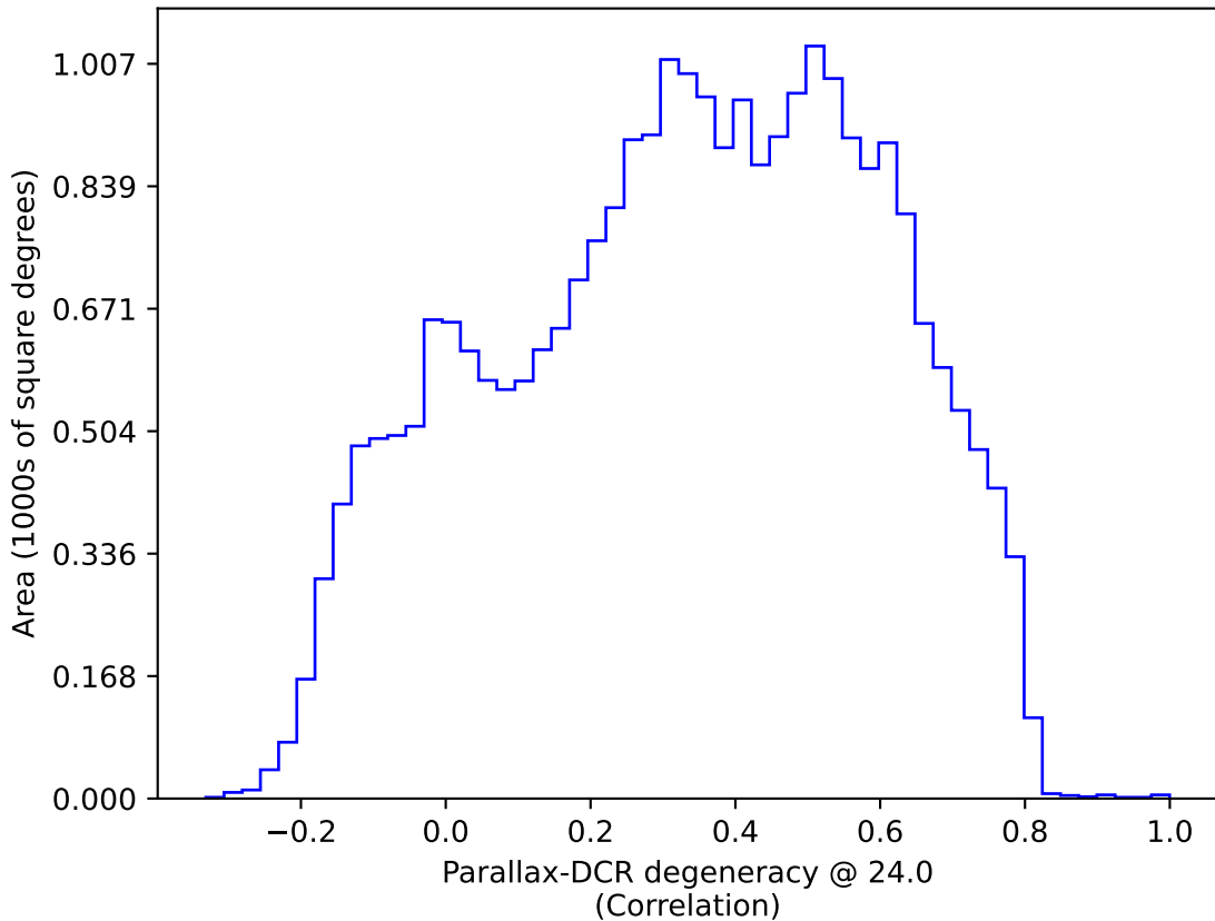
ddf_loaded_half_fl8_v3.4_10yrs All sky: Parallax-DCR degeneracy @ 24.0
