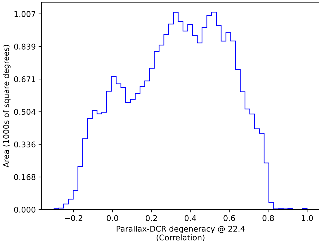
ddf_loaded_half_fl8_v3.4_10yrs All sky: Parallax-DCR degeneracy @ 22.4
