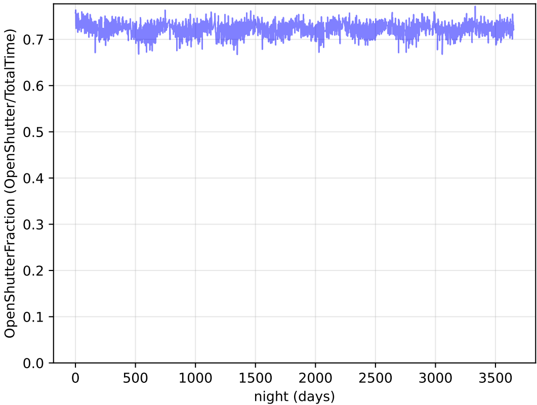
ddf_loaded_half_fl8_v3.4_10yrs Per night: OpenShutterFraction
