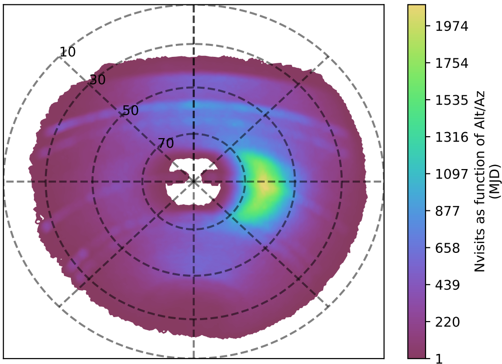
ddf_loaded_half_fl8_v3.4_10yrs y band: Nvisits as function of Alt/Az
