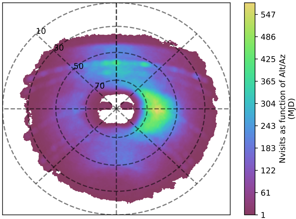
ddf_loaded_half_fl8_v3.4_10yrs u band: Nvisits as function of Alt/Az
